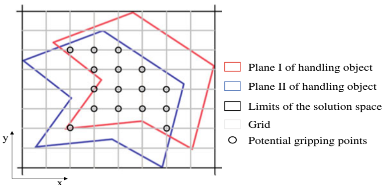
Fig. 4 Determination of potential gripping points (circles) from the two surfaces on the handling object (red, blue) with a superimposed grid in the XY-plane
