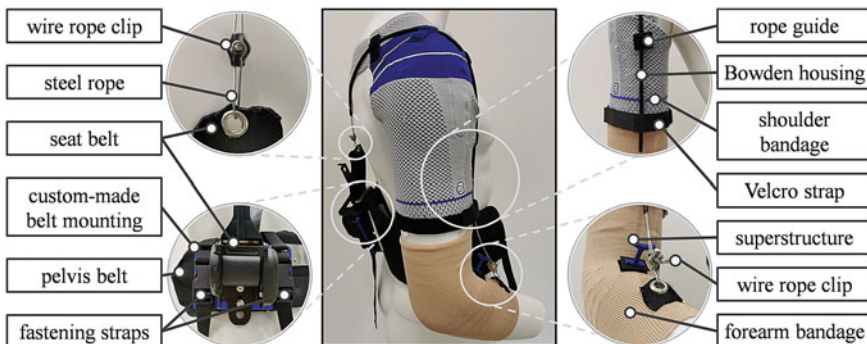
Fig. 3 Overview and central elements of the modular soft elbow support system
