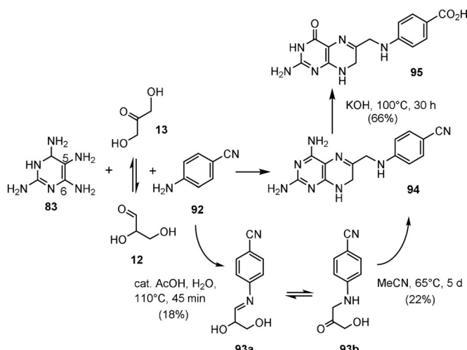
Scheme 22. A prebiotic route to simplified dihydrofolate derivative 95 . [74b]
