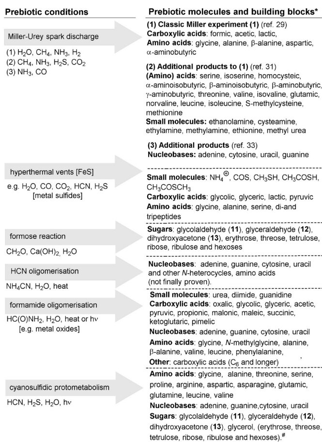
Figure 4. Overview on prebiotic molecules formed according to experimental evidence under different conditions. * The list is not comprehensive; products listed are regarded to have major relevance for current hypotheses on prebiotic evolution; for quantities and ratios refer to the original publications. # not practically demonstrated yet.
