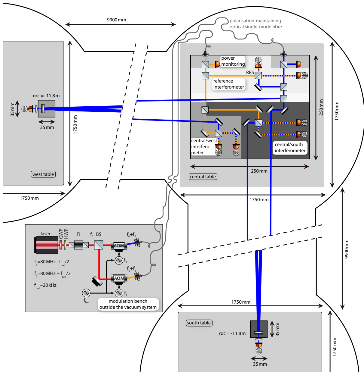
Figure 1. Schematic setup of the SPI. The reference beam is drawn in orange, the measurement beam in blue. For illustration purposes, position and size of the in-vacuum baseplates do not correspond to their real positions. Due to the small footprint of the baseplate (and overall height of 50 mm) it is still possible to place e.g. the suspended beam splitter of the SQL interferometer in the centre of the central table.
