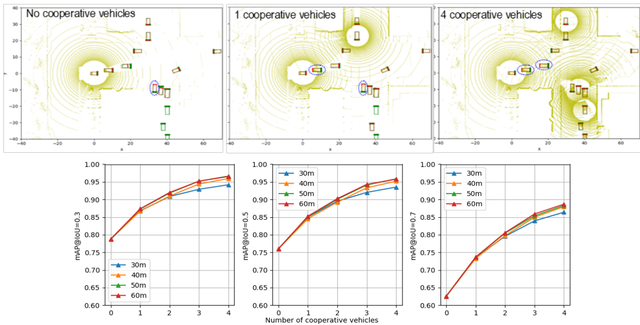
Figure 5. The vehicle detection performance of CIA-SSD. Top: detection result with/without cooperative vehicles, green indicates ground truth, red indicates predictions, the thick bar of each box tells the box orientation; Bottom: three plots show mAPs calculated with three IoU thresholds, each one shows the results with a different number of cooperative vehicles (horizontal axes, vary from 0 to 4) and communication ranges (plotted in different colors, vary from 30m to 60m)
