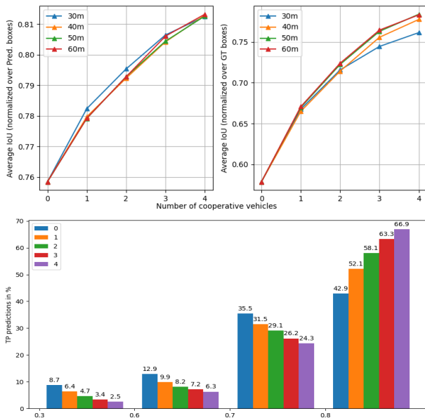
Figure 6. Influence of the number of cooperative vehicles and communication ranges on the localization accuracy (IoU) of predicted bounding boxes. Top: average IoU of all positive predicted bounding boxes with ground truth, they are normalized over the number of all true positives (left) as well as all ground truths (right); Bottom: ratios of true positive predictions in different IoU intervals for communication range 50m
