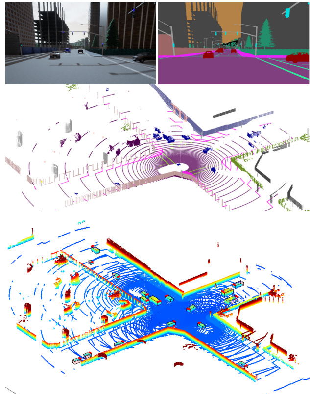
Figure 3. An example frame of the data collected by a single vehicle. Top left: RGB image; Top right: semantic segmentation label; Middle: point cloud colored by the point-wise label; Bottom: Fused point cloud data from 5 vehicles and the ground truth bounding boxes of all vehicles in the scene (height information is encoded into the point color, lines of bounding boxes are in black, the direction of bounding boxes are illustrated with a red bar on the upper front line of each box)
