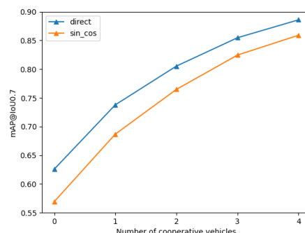
Figure 4. Performance of CIA-SSD with different bounding box target encodings at communication range 60m. The legend "direct" indicates the original encoding by the residual of ground truth angle minus the pre-defined anchor angle, where "sin_cos" means the decoupled angle encoding like PIXOR.
