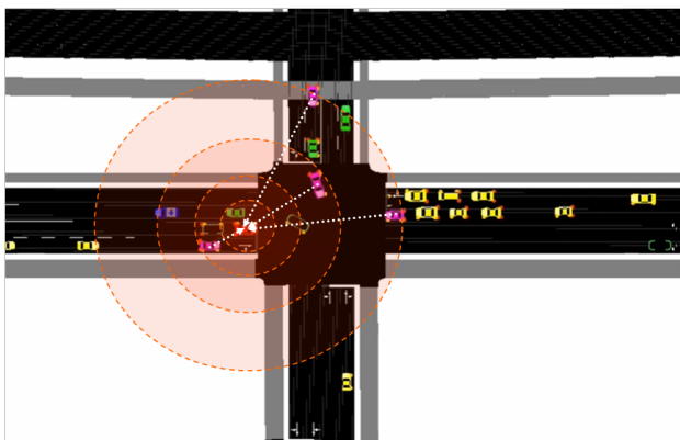
Figure 2. An example for COMAP scenario (red: ego-vehicle, magenta: data-sharing-vehicle, green: in-range-vehicles but not chosen for sharing data, yellow: not-in-range-vehicles)
