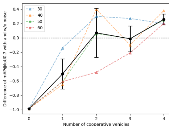
Figure 7. Influence of sensor noise on detection performance. Performance drop (mAP@IoU0.7 difference in %) of different communication ranges are plotted with the dashed line in different colors. The black solid line is the mean mAP drop of all results. Vertical bars indicate the standard deviation.
