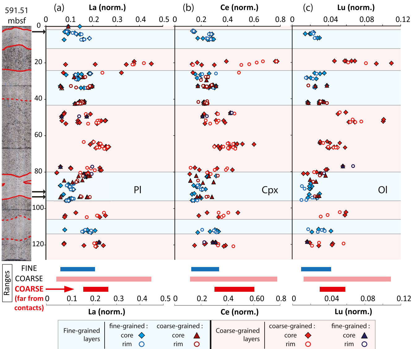
Figure 9. Depth profiles (cm from the top of the section) of (a) La in Pl, (b) Ce in Cpx, and (c) Lu in Ol, normalized to the average primitive mid-ocean ridge basalt of the Atlantis Bank area (Table S5). The compositional ranges of each lithology throughout the section are represented by the colored boxes at the bottom of the figure. The compositional range describing the coarse-grained lithology far from any lithological contacts (darker red) corresponds to the two samples from ~63 cm depth. Black arrows represent the approximate location of the finer grained areas of the fine-grained layers. Left: whole round image of section 65R5 with associated layer contacts (see Figure 2).
