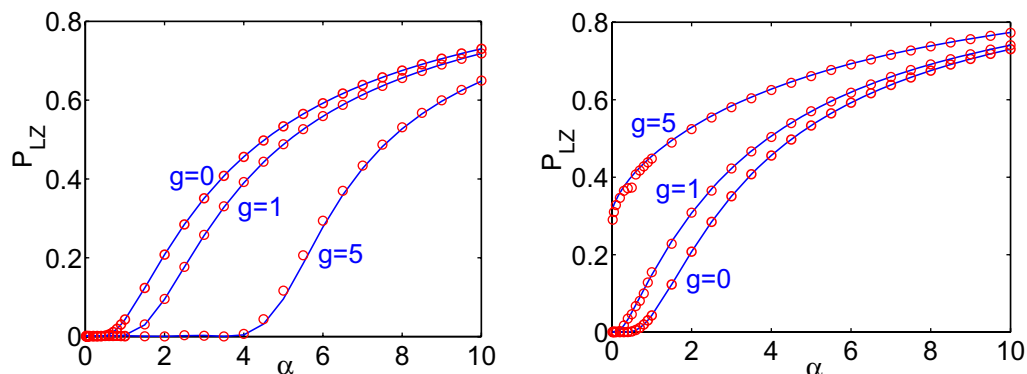
Figure 1. The Landau–Zener tunneling probability in the lower level (left) and the upper level (right) for J = 1 and g = 0, 1 and 5 . Mean-field results P_{LZ}^{\text{mf}}(\alpha) are plotted as solid blue lines and many-particle results P_{LZ}^{\text{mp}}(\alpha) for N = 50 particles as red circles.
