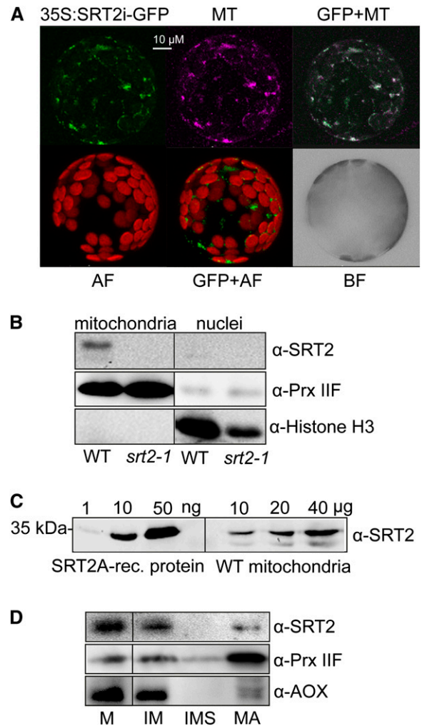
Figure 2. SRT2 -encoded proteins localize to mitochondria in Arabidopsis. A, Arabidopsis protoplasts showing GFP localizations (green) for a full-length SRT2 (plus introns)-GFP fusion construct (35S: SRT2i -GFP). Protoplasts were isolated from stable Arabidopsis transformants. Purple indicates the mitochondrial localization of MitoTracker (MT). GFP+MT indicates overlay image of 35S: SRT2i -GFP and MitoTracker; AF indicates autofluorescence of chloroplasts; and BF indicates bright-field image of protoplast. B, Western-blot analysis of SRT2 protein in mitochondrial and nuclear fractions. Antisera against PRX IIF was used as mitochondrial marker and histone H3 as nuclear marker, respectively. C, Western-blot analysis of SRT2 proteins in isolated mitochondria. Protein extracts of isolated mitochondria from wild-type (10, 20, and 40 \mu g) seedlings as well as recombinant 6 \times His-SRT2A protein (1, 10, and 50 ng) were analyzed by western blotting using SRT2 antiserum. D, Western-blot analysis of SRT2 protein in subfractionated Arabidopsis wild-type mitochondria. Ten micrograms of protein were loaded for each fraction. Antisera against Alternative Oxidase1 and PRX IIF were used as controls for the inner membrane and matrix proteins, respectively. M, Mitochondria; IM, inner mitochondrial membrane; IMS, intermembrane space; MA, matrix.
