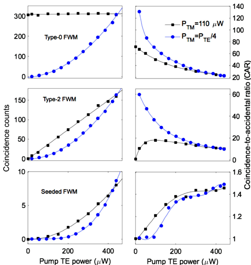
Figure 5. Power-dependent photon pair characterization. Coincidence counts acquired in 30 min (left) and CAR (right) as a function of the TE pump power for a fixed value of the TM pump power ( P_{TM} = 110 \mu W , black squares) and of the power ratio ( P_{TM} = P_{TE}/4 , blue circles). In the left panels, the coincidence rates of the type-0, type-2, and seeded FWM (top to bottom) show a constant, linear, and quadratic behavior, respectively, for P_{TM} = 110 \mu W (black), while they show quadratic, quadratic, and quartic behavior, respectively, for power scaling when P_{TM} = P_{TE}/4 . In the right panels, the lines connecting the points are for visual purposes.
