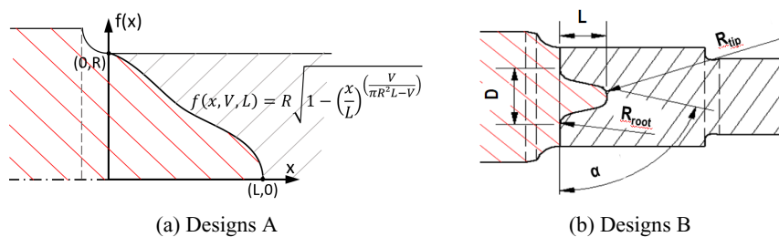
Figure 5. Design concepts
