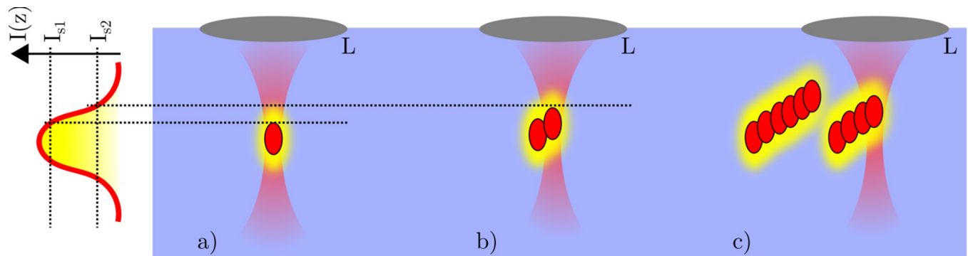
Fig 10. Schematically representation to illustrate the cause of formation of step-like structures inside a transparent hydrogel (blue). Shown is the intensity profile of the laser beam (red) due to focusing through a lens L. a) depicts the optical breakdown (red ellipse) after exceeding the damage threshold. Additionally, a chemical material decomposition (yellow ellipse) due to the laser intensity reduces the materials damage threshold. Hence, b) shows the exceeding of damage threshold at IS2, which leads to a displaced optical breakdown for the second pulse. Since the variation of the materials damage threshold is reduced by increasing distance from the original focus (yellow shading), this results in the step-like structures as shown in c).
