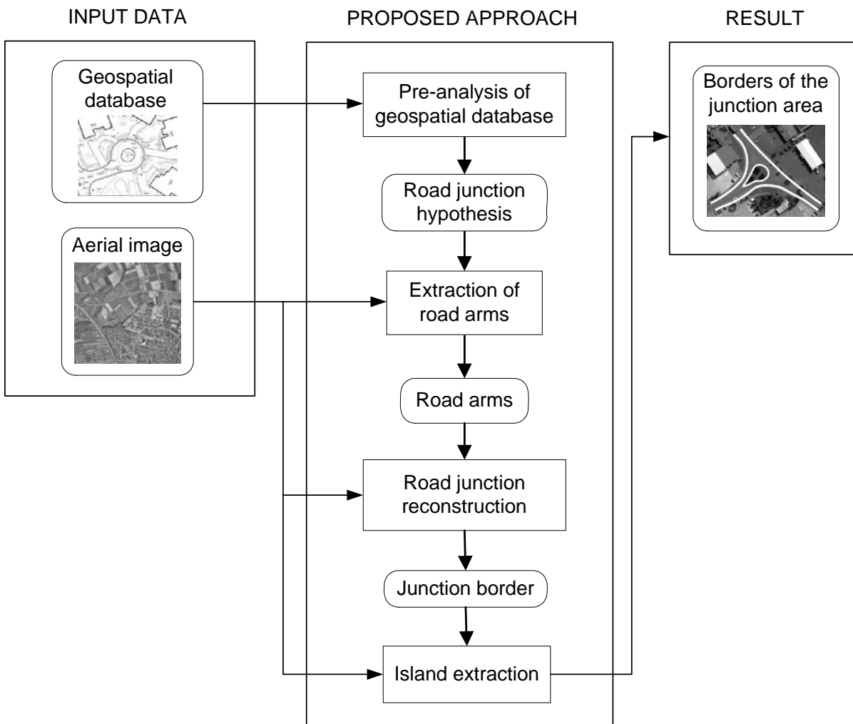
Figure 3-3: Proposed approach organization
