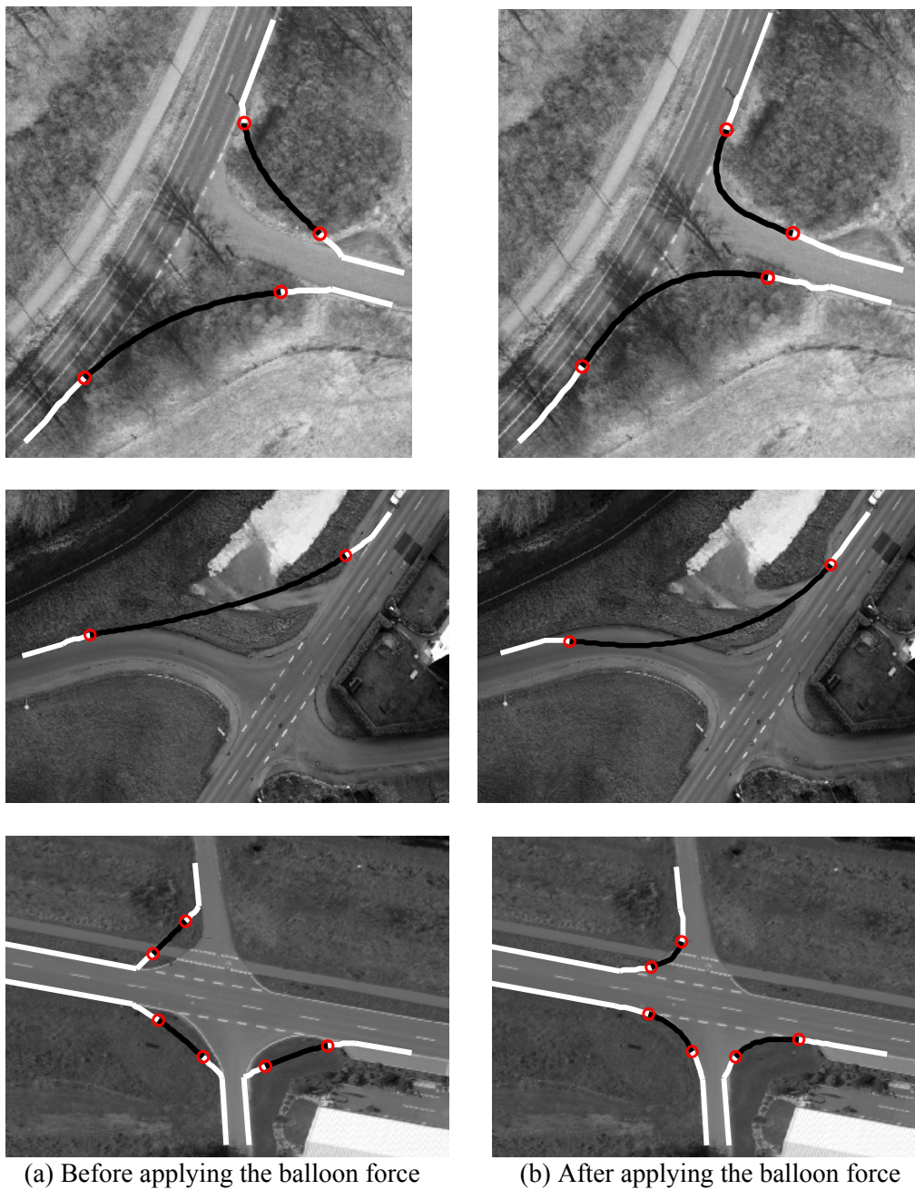
Figure 3-17 : (a) Snake optimization before the balloon force is applied. Active curves (white) and the passive part (black) are approximately straight. (b) The effect of the balloon force on the passive and active parts is shown after the balloon force is applied for the first time.
