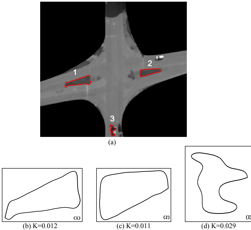
Figure 3-33: Illustration of the curvature constraint. (a) Islands labeled with numbers before applying curvature constraint. (b), (c) and (d) display the approximated curves 1, 2 and 3 and their computed mean curvature. The closed curve in (d) is not considered as an island as its mean curvature value is too high.
