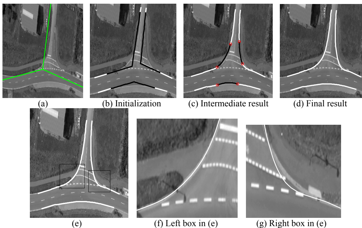
Figure 4-4: Illustrating the effect of road markings. (a) Vector data. (b) Initial snakes in black. (c) Snakes during evolution. (d) Extracted junction. Both scenes in (f) and (g) contain similar contrast and road markings. However, a better result is seen in (f). The reason is that, in (g), the warning lines are closer to each other involving more snake vertices. As a result, the curve is entered the junction area. In (f), stop and warning lines are close to each other at the top, however, they don't disturb the snake optimization because they are approximately perpendicular to the snake's movement direction.
