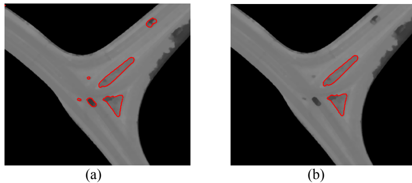
Figure 3-31: (a) Closed curves are retained as island candidates. (b) Two cars having areas of 13 and 11 m 2 are eliminated. The remaining islands have areas of 67 and 52 m 2 .
