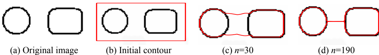
Figure 2-5: (a) Original image. (b) Initial closed contour situated around two objects. (c) Intermediate contour during the evolution. (d) Final curve that is converged to boundaries. It is proved that the snake model can not naturally change its topology during the evolution process since the final contour has captured only one object.
