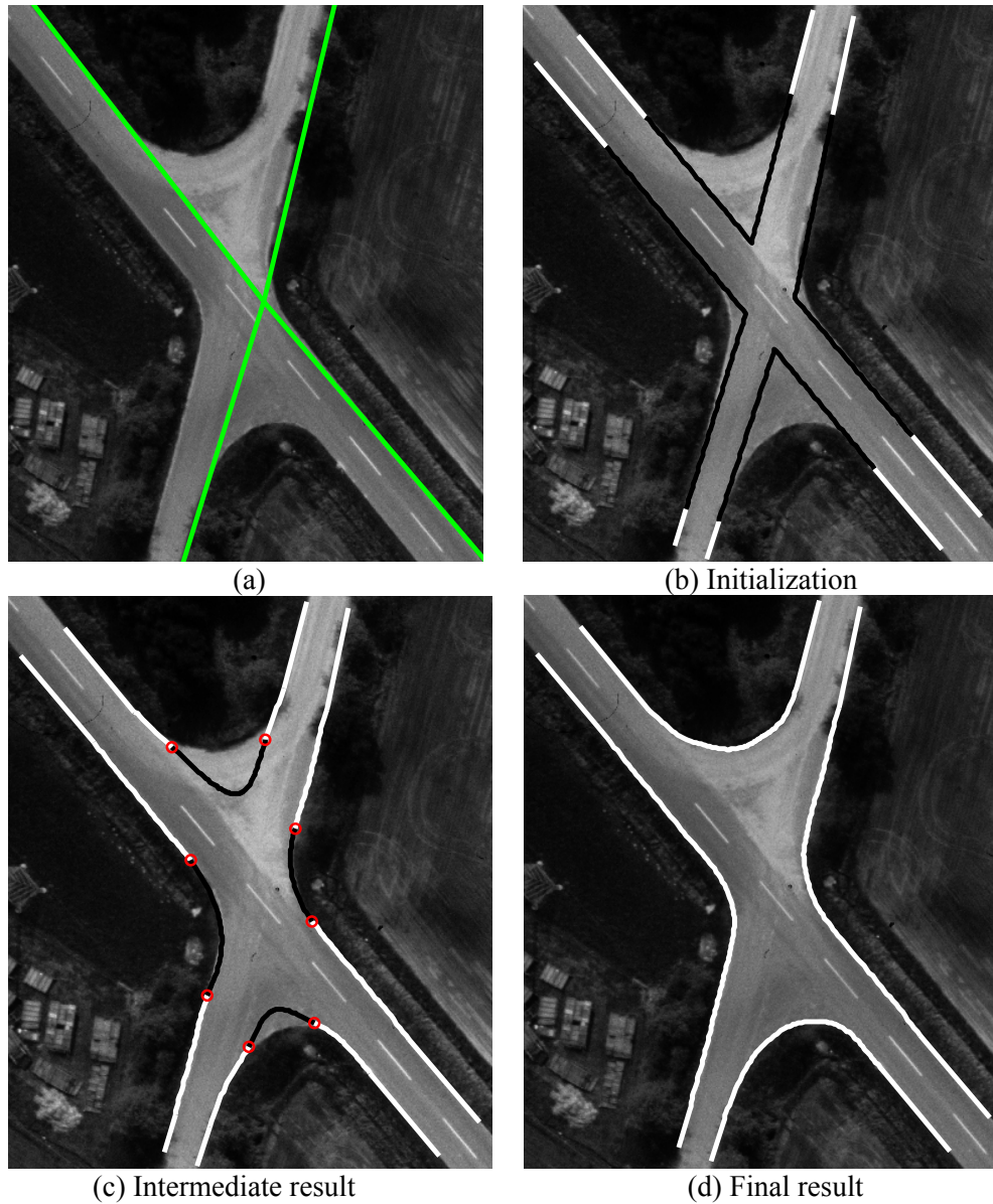
Figure 4-14: (a) Vector data. In (b), initial curves at the top and bottom are very far away from the borders. In (c), the passive part of the ziplock snake (black) at the top is much farther from the junction border than that in the bottom, because different radiometric properties at the top hinder the snake motion. Therefore, a higher number of iterations is needed to recover the border. (d) Extracted junction.
