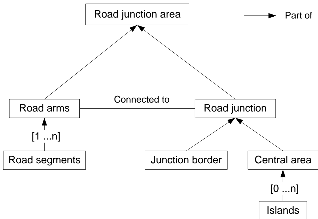
Figure 3-2: Road junction model
