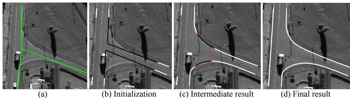
Figure 4-12: Shows the case in which shadows from different sources exist. (a) Vector data. (b) Initial snakes in black and road arms in white. (c) Snakes during evolution. (d) The final result indicates that shadows can be overcome by our snake method.
