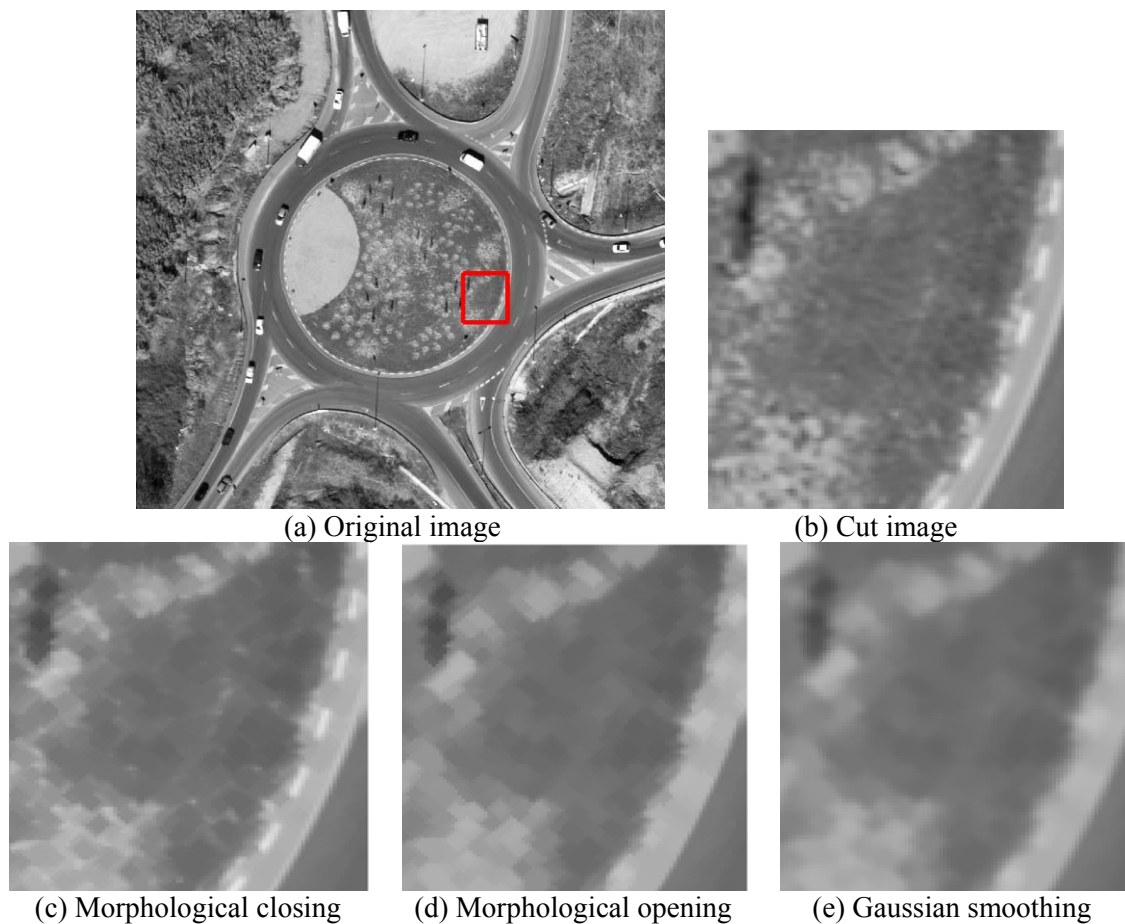
Figure 3-39: Illustrating preprocessing steps. (a) Original image. (b) A cut-out marked in the red box in (a). In (c) and (d), a disk structuring element of size 2 is used for the morphological operations. In (e), Gaussian smoothing with disk structuring element of size 3 and standard deviation 2 is applied.
