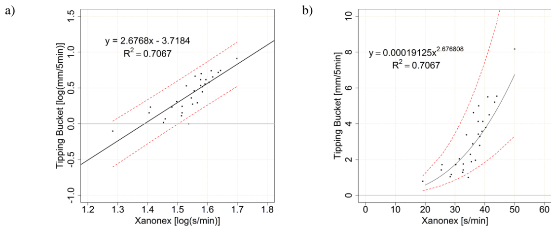
Fig. 5. (a) Xanonex log transformed W-R relationship (b) Xanonex W-R relationship after Eq. 5; the red lines illustrate the 95% prediction limits
