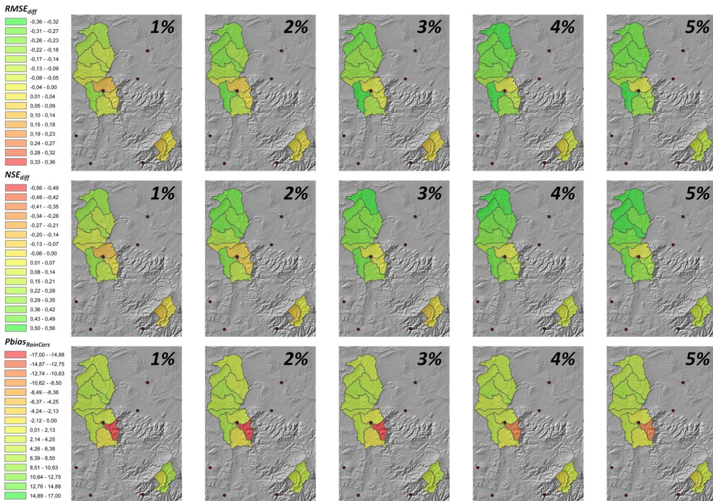
Fig. 8. Areal rainfall estimation evaluation using RCs for the Nette and Sieber catchment. The green colour for RMSE_{diff} and NSE_{diff} illustrate the improvement of the areal rainfall estimation quality when RCs are used compared with when only rain gauges are considered.
