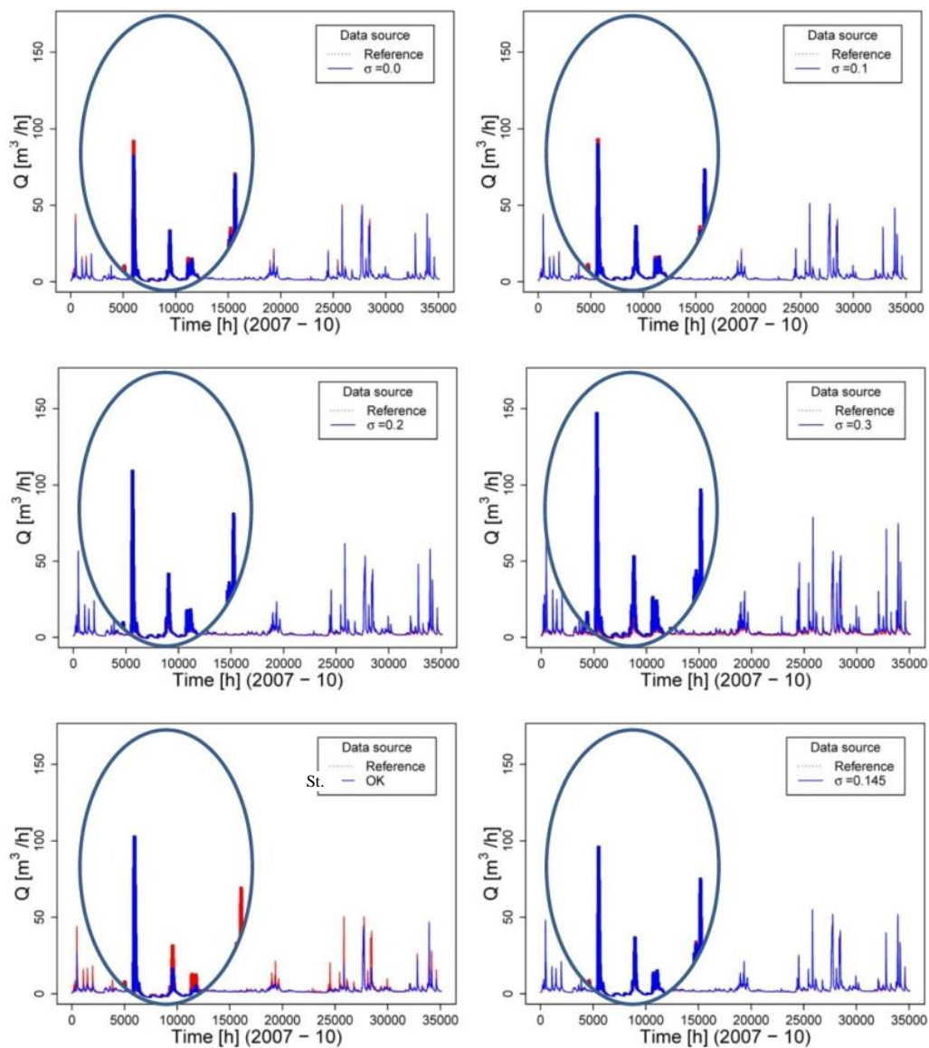
5 Fig. 9. Discharge simulation using different sources of data for the Nette catchment. For RCs only 5% scenario is considered.
