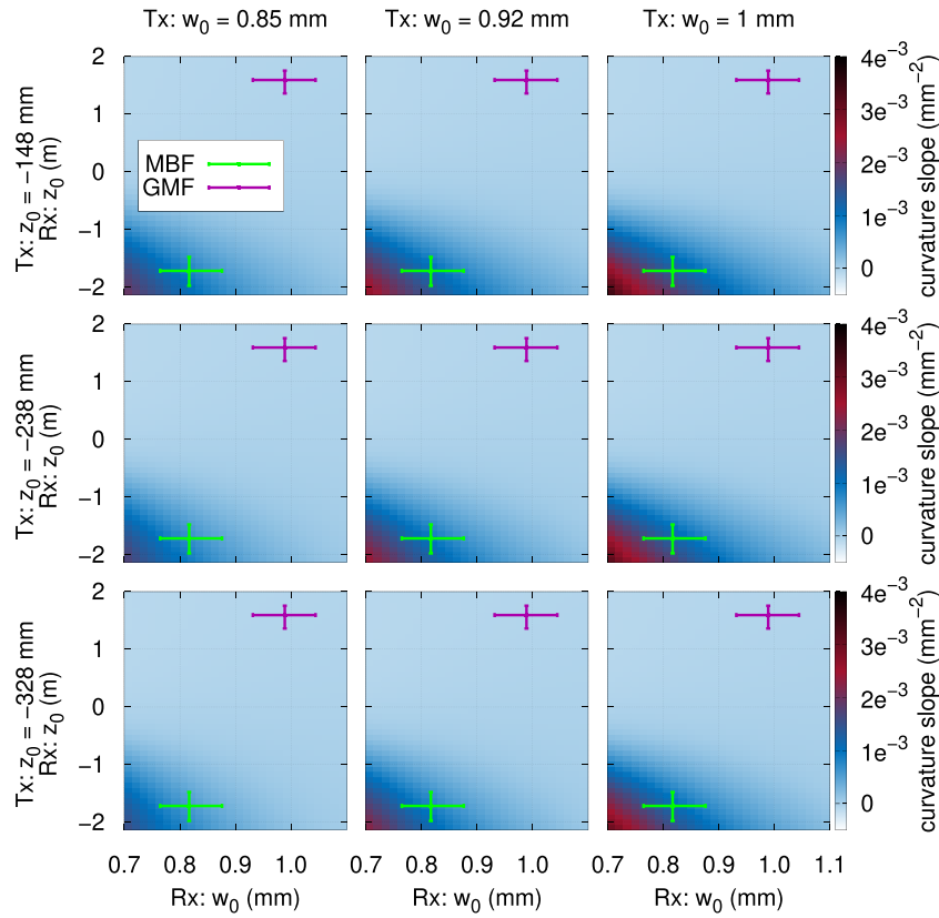
Figure 17. Simulated beam curvature difference slope at the optimal QPD position behind the two-lens imaging system, corresponding to figure 15. A clear correlation between the TTL coupling and the curvature difference slope can be observed.
