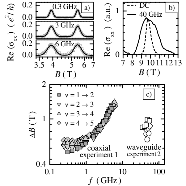
FIG. 1. (a) Conductivity of sample 1 measured in the coaxial setup. Here shown are the conductivity peaks at the \nu = 4 \rightarrow 3 and \nu = 3 \rightarrow 2 plateau transition. (b) Conductivity of sample 2 at the \nu = 2 \rightarrow 1 transition, measured in the waveguide reflection setup for very high frequencies and in a classical Hall setup for dc. (c) Frequency dependence of the width of the QH plateau transitions, measured for \nu > 2 as full width and for \nu = 2 \rightarrow 1 as half width at half maximum [24,26]. For the waveguide experiment, different symbols denote different samples from the same wafer or different cooldown cycles with slightly different carrier densities.
