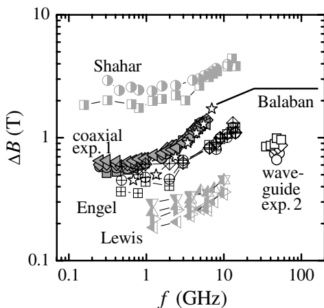
FIG. 2. Comparison of the transition width vs frequency for all experiments [10,19–25]. Multiple symbols for the same experiment denote different samples or cooldowns (waveguide), transitions (coaxial, Lewis), or temperatures (Engel, Lewis, Shahar) as presented in Table I.
