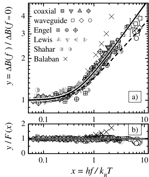
FIG. 3. (a) Normalized plateau transition width y = \Delta B(f, T) / \Delta B(f \approx 0, T) vs x = hf/k_B T for all data presented in Table I and Fig. 2. The solid line results from a fit of F(x) = [1 + (\alpha x)^2]^{\kappa/2} [Eq. (3)] to all data except those for f > 20 GHz and the Balaban experiment ( \alpha \approx 2 , \kappa = 0.5 \pm 0.1 ). The dashed line depicts a reduced \kappa = 0.4 . (b) Rescaling of y = \Delta B(f, T) / \Delta B(f \approx 0, T) by the scaling function F(x) allows one to judge the quality of scaling.
