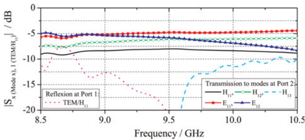
Fig. 14. Scattering parameters of the stepped transition.
