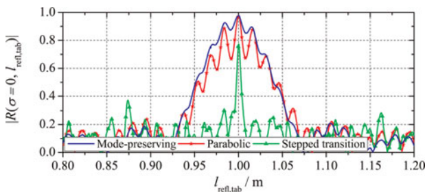
Fig. 16. |R(\sigma = 0, l_{ref,tab})| at l_{ref} = 1.0 m for three different transitions.
