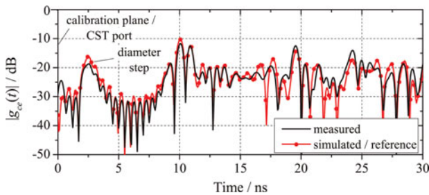
Fig. 15. Measured and simulated envelopes for l_{ref} = l_{ref,tab} = 1.0 m.
