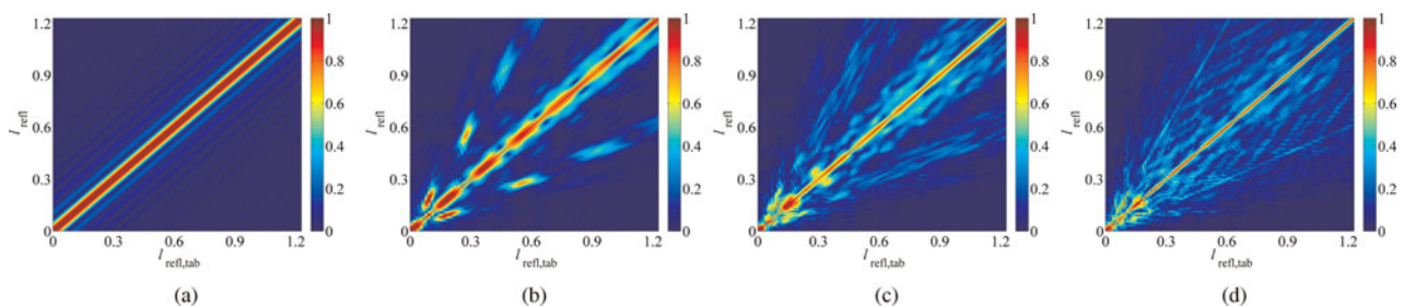
Fig. 7. |R(\sigma = 0, l_{refl,tab})| for all l_{refl,tab} and l_{refl} in case of one to four modes: (a) one mode, (b) two modes, (c) three modes and, (d) four modes.
