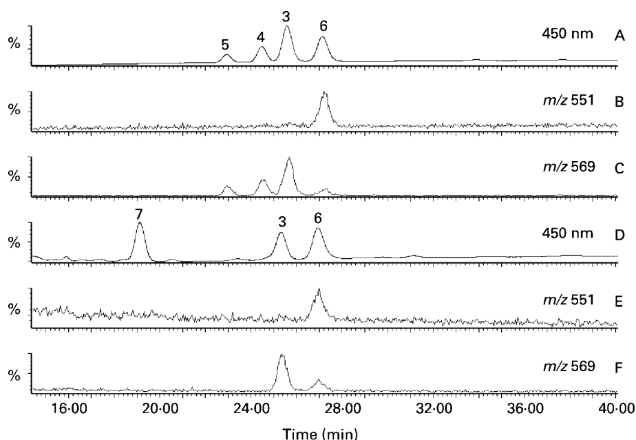
Fig. 2. Liquid chromatography (LC)–atmospheric pressure chemical ionisation (APCI)–MS analysis (extended sections) of a standard mixture (trace A) of zeaxanthin stereoisomers (3R,3'R (peak 3), 3R,3'S (peak 4) and 3S,3'S (peak 5)) and 3R,3'R,6'R-lutein (peak 6), and mass traces for lutein ( m/z 551) (trace B) and zeaxanthin ( m/z 569) (trace C). Trace D corresponds to the LC–APCI–MS chromatogram (diode array detector, 450 nm) of a pooled plasma sample after ingestion of 3R,3'R-zeaxanthin palmitate (3R,3'R-zeaxanthin (peak 3), 3R,3'R,6'R-lutein (peak 6), and lycopene (peak 7) and the corresponding mass traces for lutein ( m/z 551) (trace E) and zeaxanthin ( m/z 569) (trace F).
