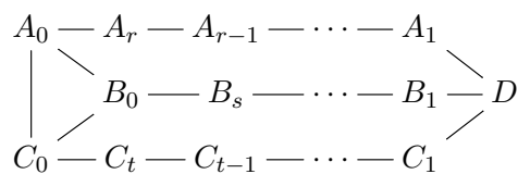
FIGURE 1. Graph of G = (V, E) .
