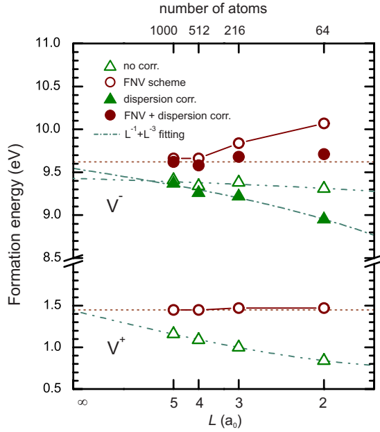
FIG. 2. (Color online) Demonstration of the correction schemes for the formation energies of the Cl vacancy in the +1 and -1 charge states (in Cl-rich limit) with respect to the reciprocal supercell lattice constant L^{-1} . The calculations were performed with the GGA-PBE functional without structural relaxations.
