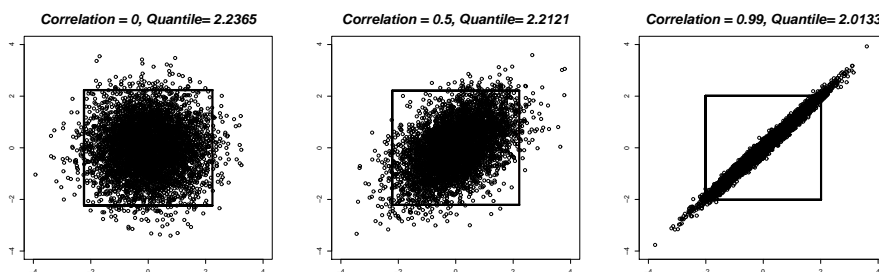
FIG 1. Two-sided equicoordinate quantiles of different bivariate N(\mathbf{0}, \mathbf{I}_2 + \rho(\mathbf{1}_2\mathbf{1}'_2 - \mathbf{I}_2)) distributions with different correlations \rho : \rho = 0 (left), \rho = 0.5 (middle) and \rho = 0.99 (right).
