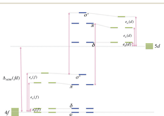
Fig. 2 Representation of the AOM parameters adjusted from the interaction of a lanthanide ion with one ligand. The first order energy splitting of the 4f and 5d orbitals is presented in green and the second order energy splitting in blue.
