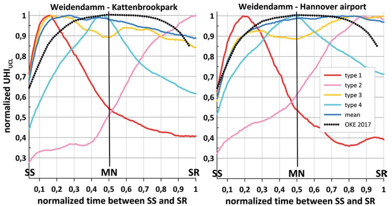
Figure 6: Normalized nocturnal evolution of canopy layer urban heat island (UHI UCL ) types for the difference in rural-urban air temperatures (WD-K) (left) and WD-HAJ (right). The dotted line represents the idealized expectation according to Oke et al. (2017).
