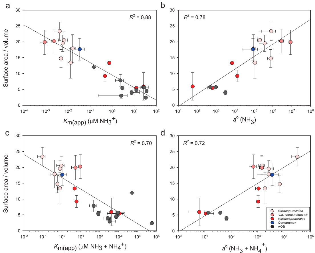
Fig. 5 Logarithmic correlation of the substrate affinity ( K_{m(\text{app})} ) and specific substrate affinity ( a^\circ ) with the cellular surface area to volume ratio of ammonia-oxidizing microorganisms (AOM). All K_{m(\text{app})} (a, c) and a^\circ (b, d) values correspond to values presented in Fig. 2. The surface area to volume (SA/V) ratio calculations for each AOM are provided in Table S4. Data for AOA (red), comammox (blue), and AOB (black) are shown. The three different gradations of red differentiate three distinct AOA phylogenetic lineages. The error bars represent the standard deviation of replicate kinetic experiments or SA/V ratio measurements of each AOM strain. The logarithmic correlation ( R^2 ) value was calculated from the average values of each AOM and is presented on a semi-log axis.
