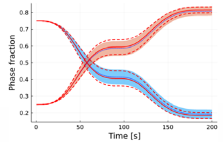
Evolution of the expectation plus/minus the standard deviation of volume fractions during phase transformations.
