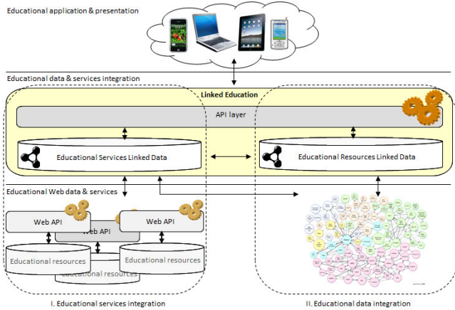
Figure 1. Approach overview
