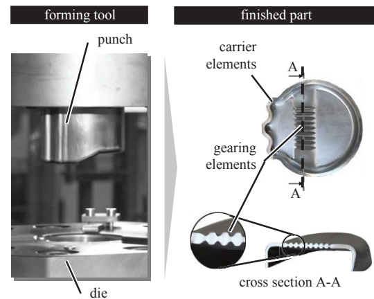
Fig. 3. Forming tool and finished part
