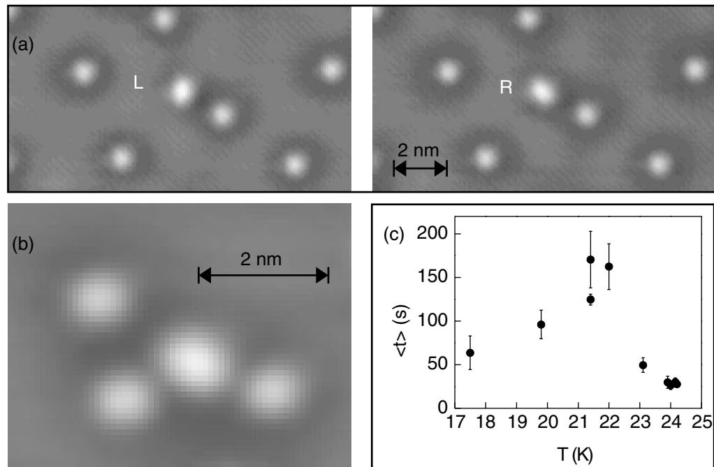
Figure 7. Influence of adatoms on dimer rotation ( \Delta t = 100 s, 203 mV, 0.43 nA). (a) T = 21 K, closest distance from dimer to adatom \Delta d = 1.68 nm, dimer positions: LRRRRLLLLLRLRLLRRRLLLLLLR. See movie 3 and movie 4 . (b) T = 17 K, \Delta d = 1.7, 1.21 and 1.36 nm, consecutive dimer positions: RRRHHLRRHLLLHLLLHLLH. See movie 5 . (c) Average residence time ( \langle t \rangle ) of a dimer in one of three equivalent positions during rotation versus temperature T .
