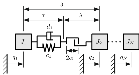
Figure 2: Backlash between the first and second mass. The system is considered rotary.
