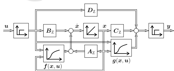
Figure 4: State space representation of the construction kit modelling with linear and non-linear part.
