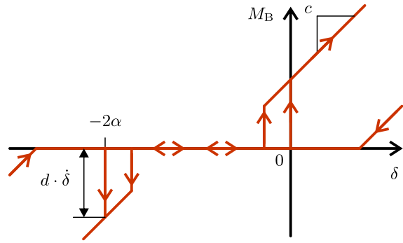
Figure 3: Hysteresis loop of the spring damper element with backlash.
